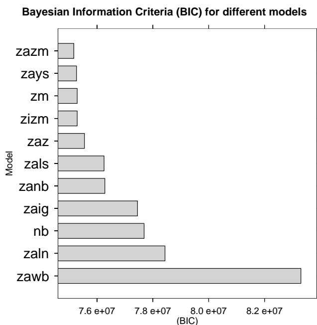
Figure 6: User-level BIC values (lower is better): Zero-altered models (ZA..) do better than zero-inflated (ZI..) or unadjusted (e.g. ZM). Within the zero-adjusted set, Zipf-Mandelbrot does the best.
